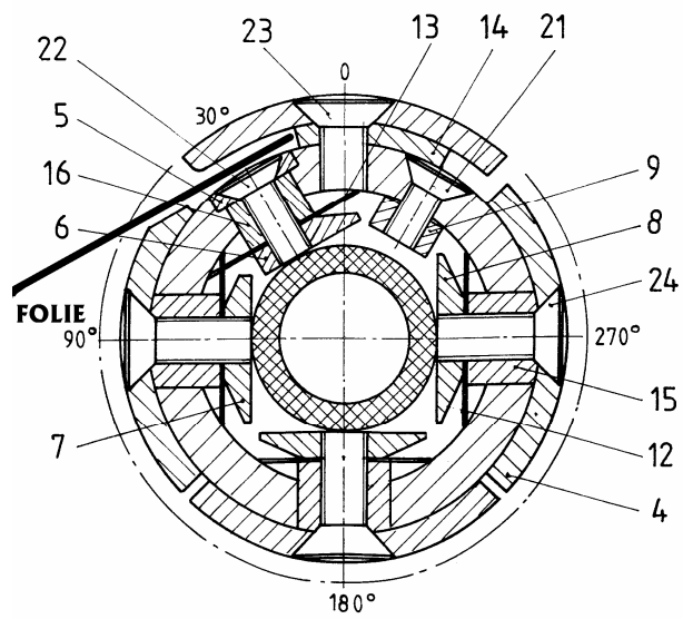
Drawing 1: The web material, titled with „Folie“, must be inserted in the slit between fixed leaf (23) and gripping ledge (22).
